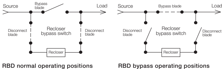
RBD normal operating positions
