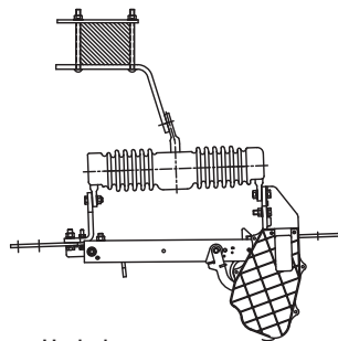
Underhung
