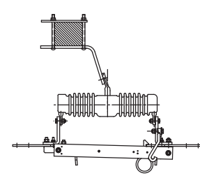
Underhung
