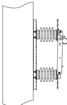
Polemount
