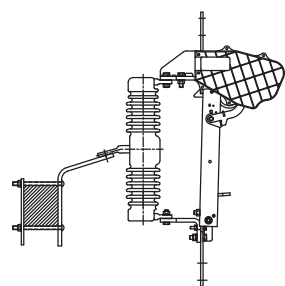
Extended angle
